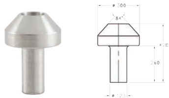
LM-II-L Nozzle Assembly Diamond Sapphire
