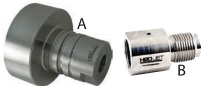
Check Valve 1.5 GPM 60k Main Body 1.5 GPM (A) Outlet Body (B)
