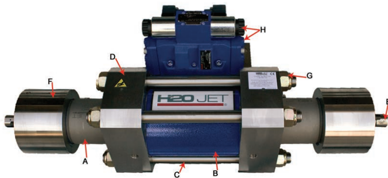
1.5 GPM 60k Long Block Intensifier 60k Electric Shift, Hi-Load & Manifold
