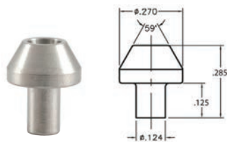
LS-II Nozzle Assembly Diamond Sapphire
